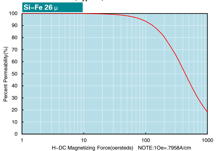
DC-Bias Curves(Typical)
